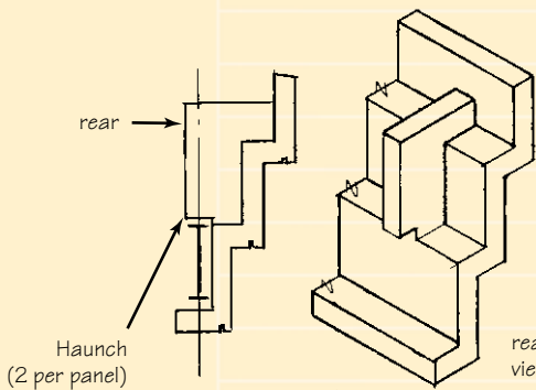
Fig. 3-7A Special Haunch on Panel
