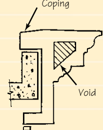
Fig. 3-6 with Coping and Void
